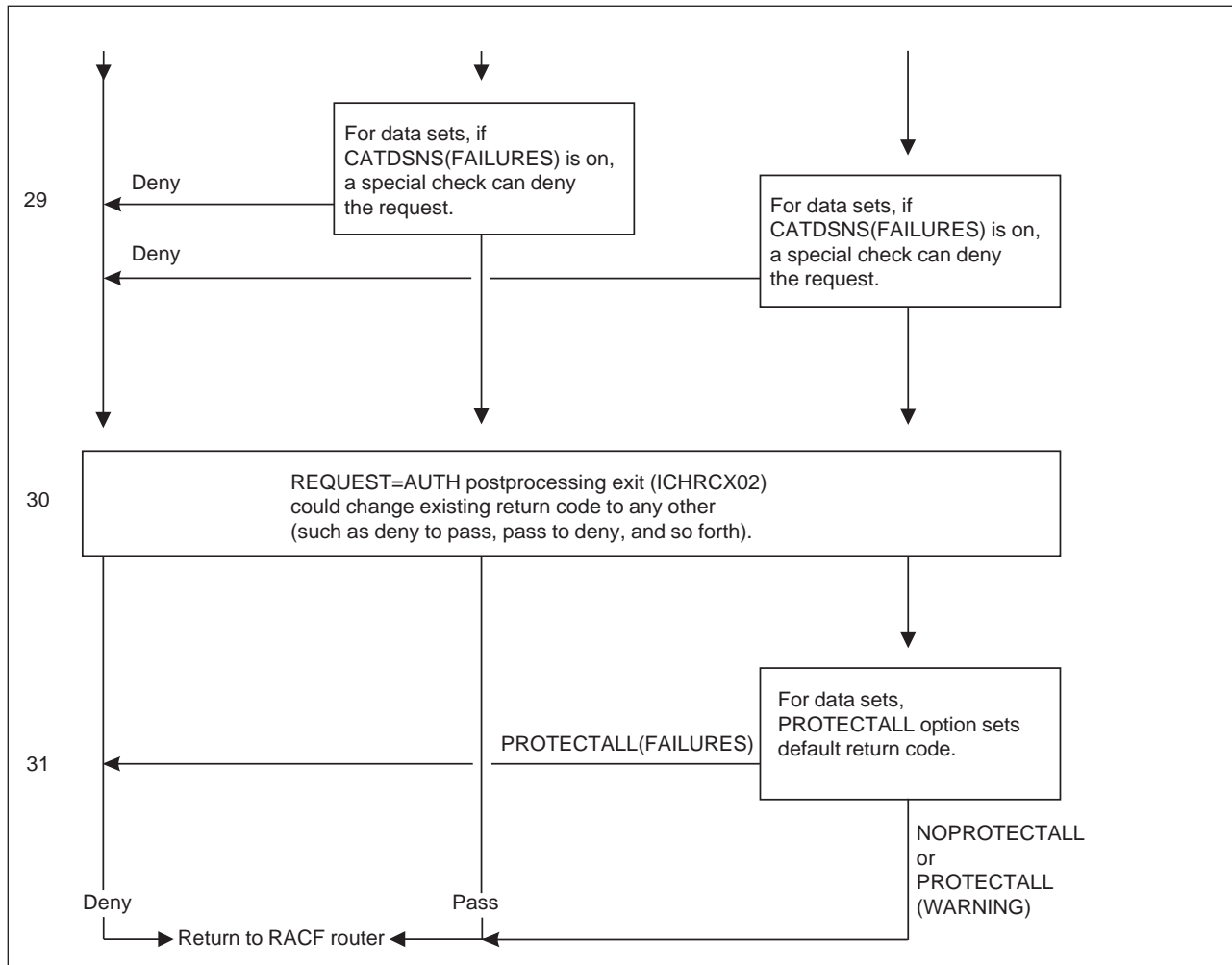
Figure 75. Process Flow of RACF Authorization Checking (Part 3 of 3)
