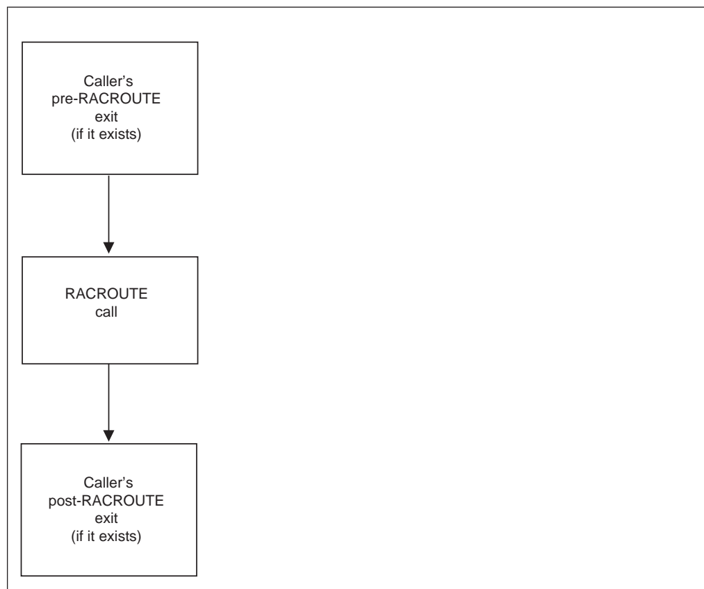
Figure 72. Process Flow of Callers of RACF for RACROUTE REQUEST=AUTH Requests
