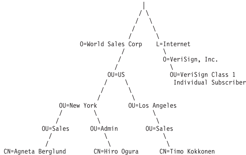
Figure 61. Example of an X.500 Directory Information Tree
