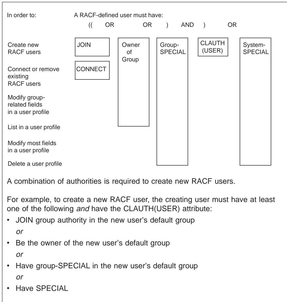
Figure 7. Delegating Authority (User Profiles)
