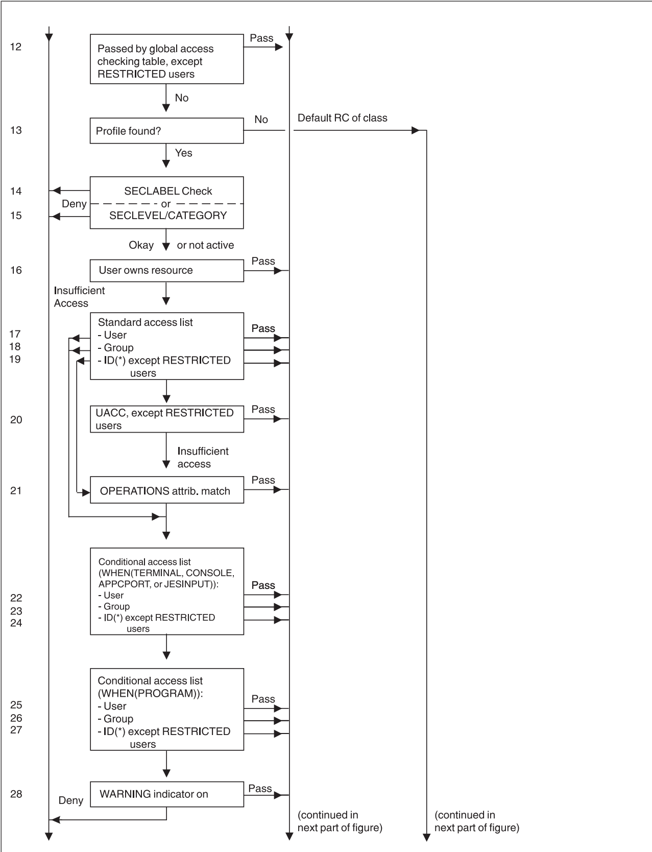
Figure 75. Process Flow of RACF Authorization Checking (Part 2 of 3)
