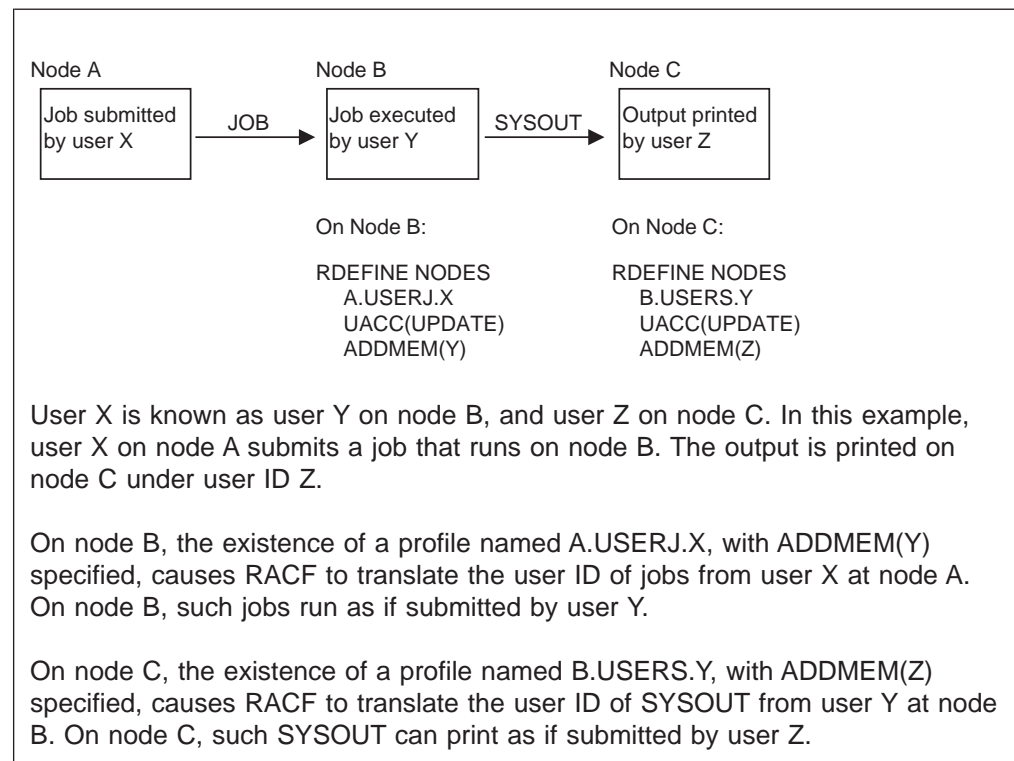
Figure 52. Example: Simple NJE User Translation
