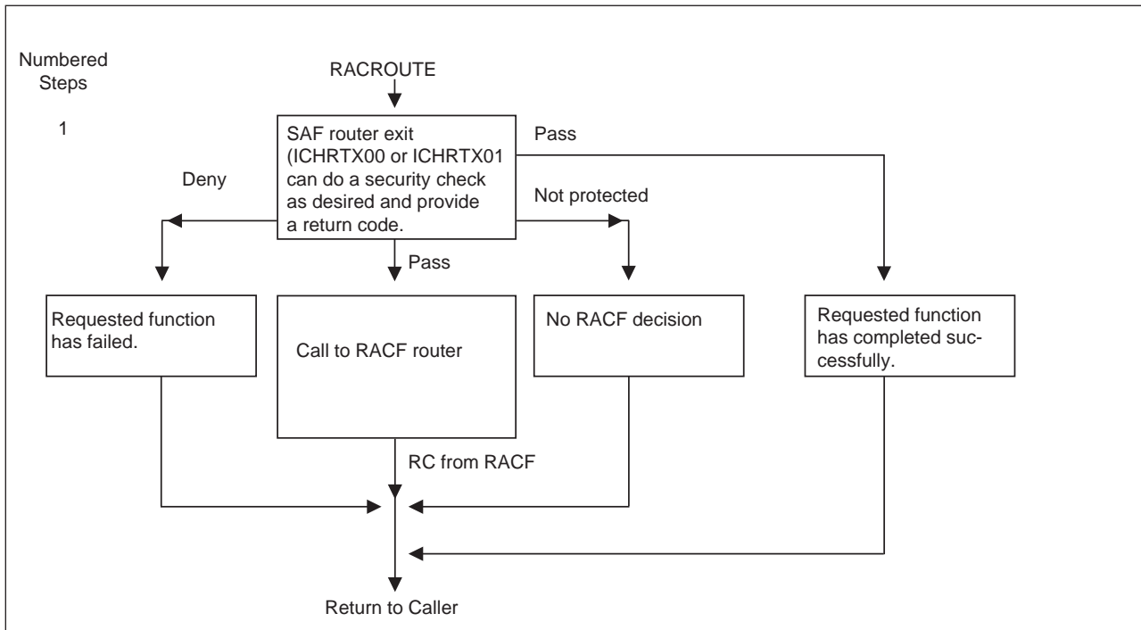
Figure 73. Process Flow of SAF Router for RACROUTE REQUEST=AUTH Requests
