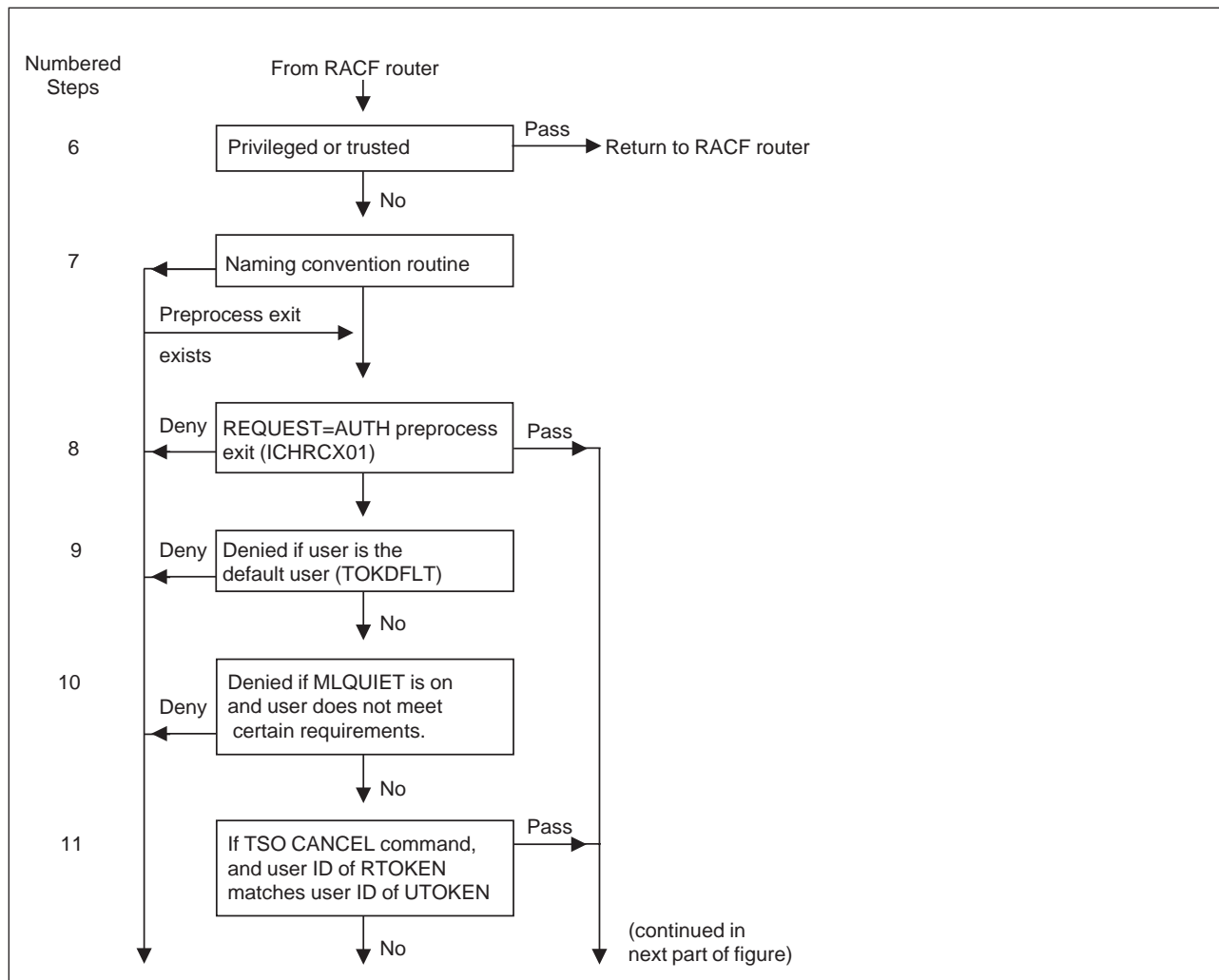
Figure 75. Process Flow of RACF Authorization Checking (Part 1 of 3)
