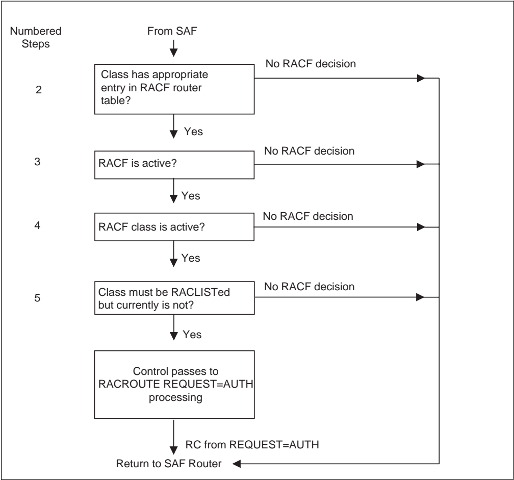
Figure 74. Process Flow of RACF Router
